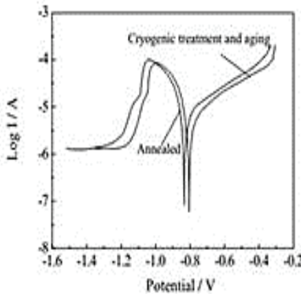
Figure 8. Potentiodynamic test of untreated and treated LC4 (Al-Zn-Mg-Cu).
