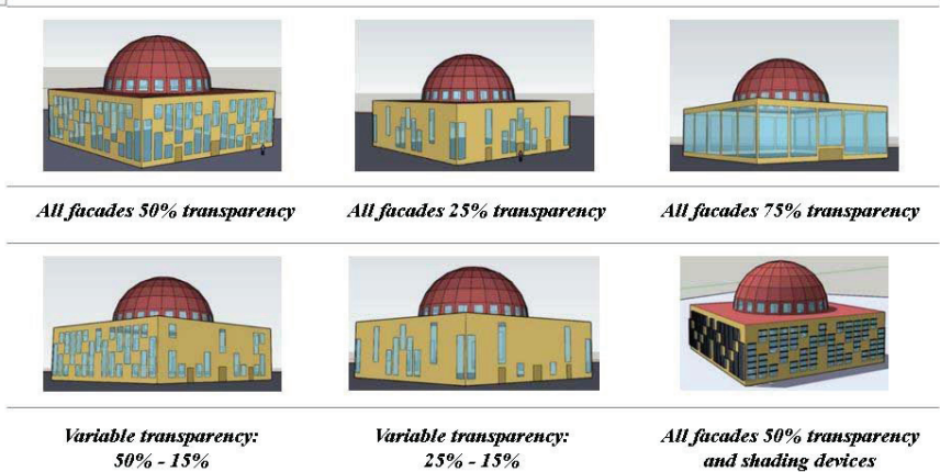
Figure 6: Different facade scenarios. (Zorer Gedik et al., 2021, p. 7)
