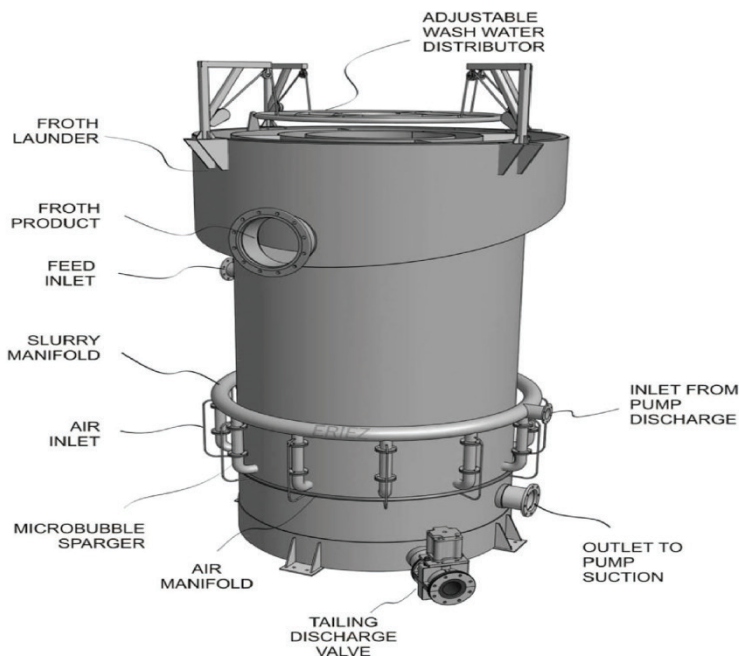
Figure 3. Column Flotation Tank with SlamJet sparging (Eriez Company)[23]
