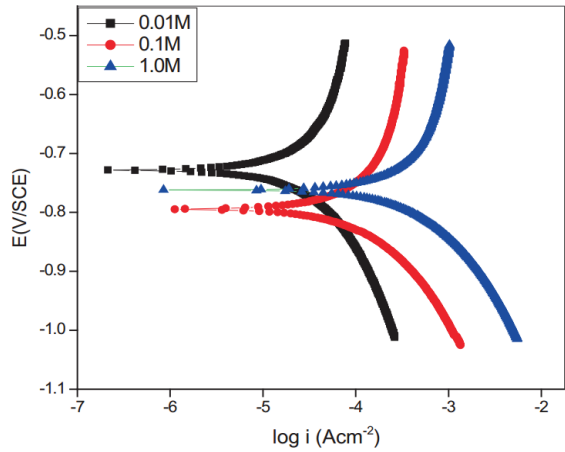
Figure 10. Anodic curve of 6063 alloy in different concentration of H_3PO_4 at 30 °C (Deepa & Padmalatha, 2017) .
