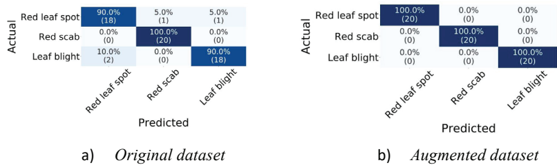
Figure 5. Confusion matrices for original and augmented dataset
