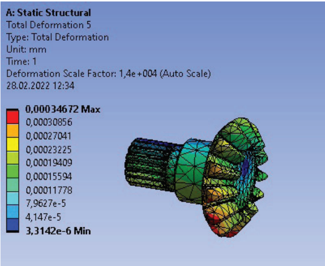
Figure 12 Deformation axle gear
