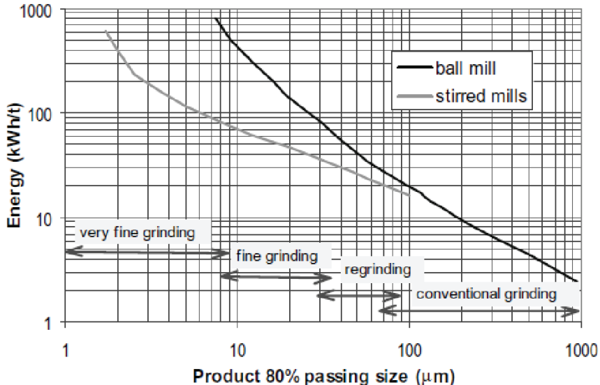
Figure 2. The micronized grinding size change vs energy limits in ball milling models [5-6]
