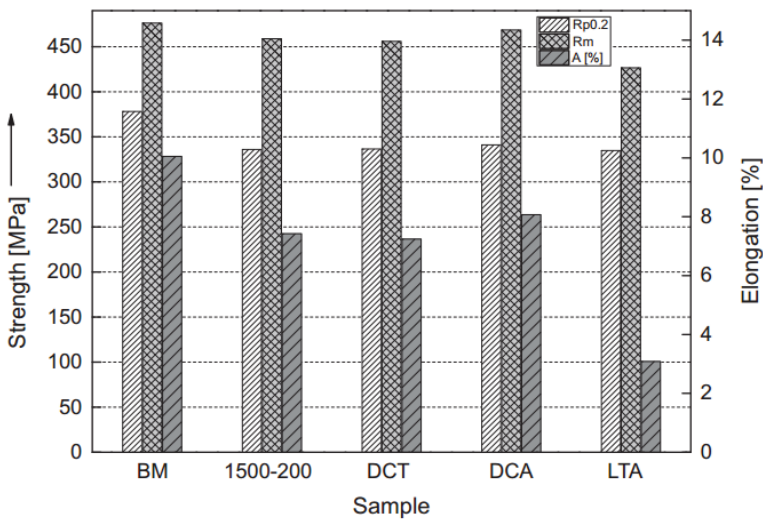
Figure 13. Tensile properties of 2024 with different heat treatment (Wang et al., 2014).
