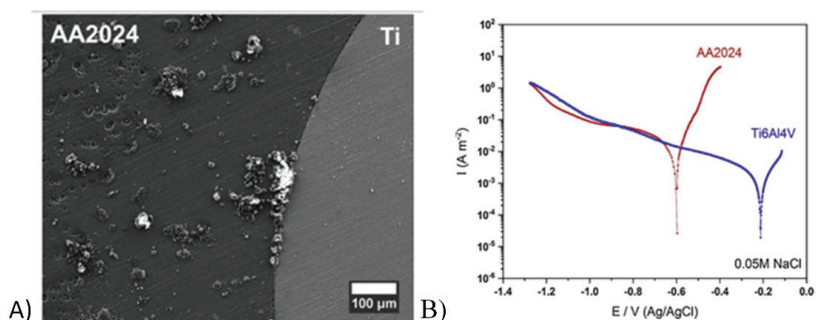
Figure 9. AA2024-Ti galvanic couple A) after 25 h of immersion and B) potentiodynamic curves in 0.05 M NaCl (Snihirova et al., 2019).
