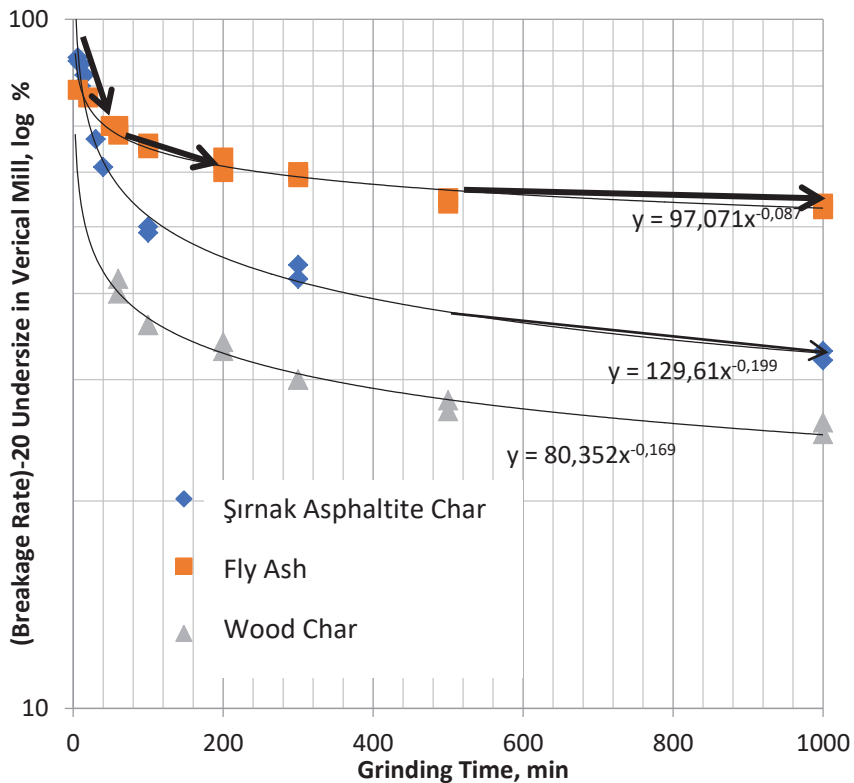
Figure 10. Ultrafine Grinding rate Change over the microwave radiated samples of char below 20 micron .
