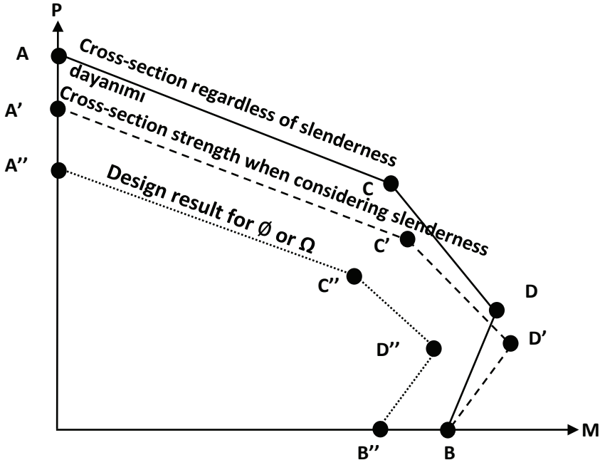
Figure-2. ÇYTHYE-2018 (Figure 12.7) Interaction diagram developed for CFST elements
