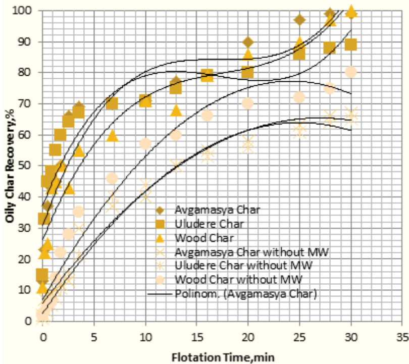
Figure 7. Char carrier cycling column flotation washing results
