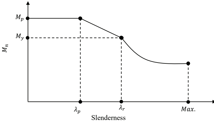
Figure-1. ÇYTHYE-2018 (Figure 12.5), characteristic bending moment strength in CFSTs
