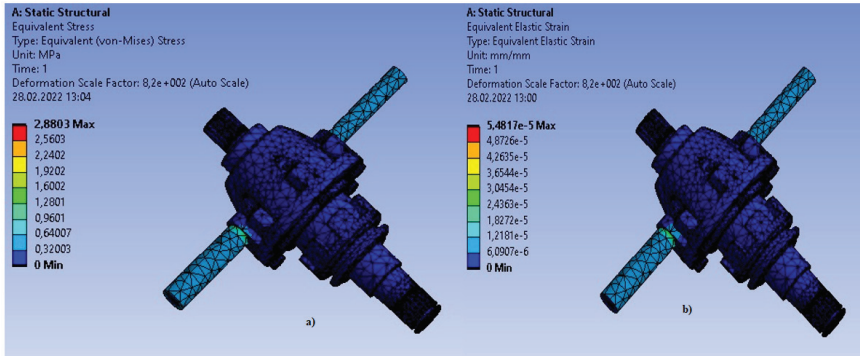
Figure 14 a) Equivalent Stress Analysis b) Equivalent Elastic Strain
