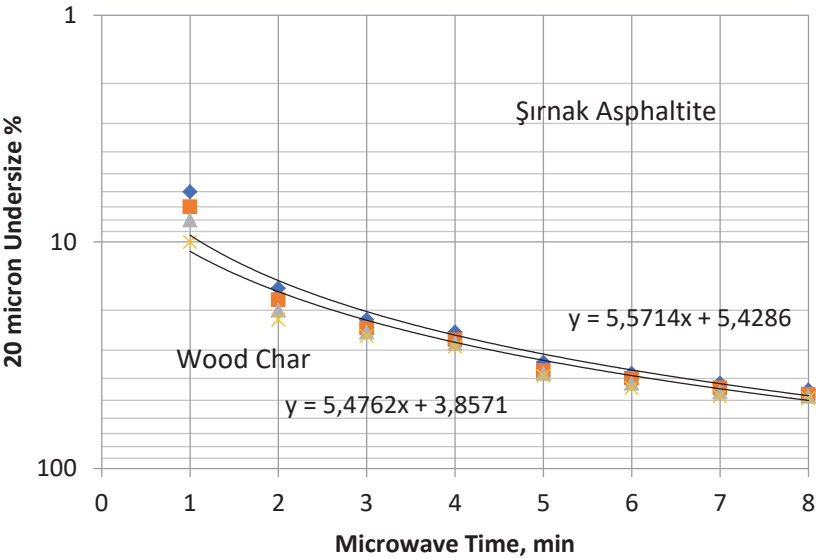
Figure 8. The Bij Breakage rate change for -20micron finer grinding at 30 min.
