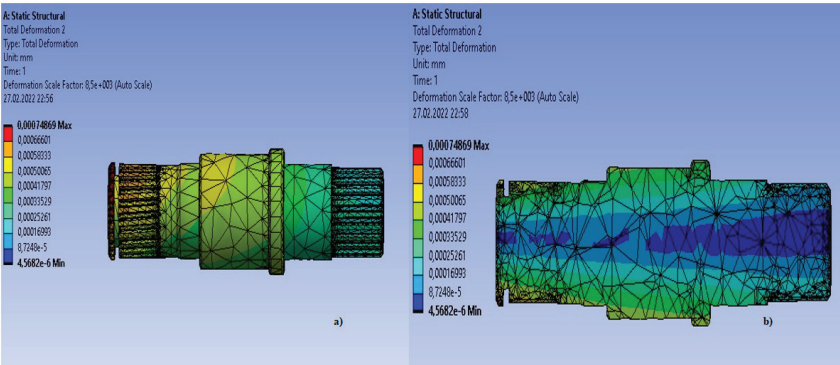
Figure 11 Deformation a) axle shaft b) axle shaft section
