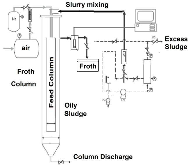
Figure 4 Cycling column flotation equipment and Froth generation schematic views
