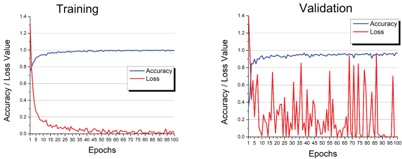
Figure 3. Accuracy and loss curves of training and validation
