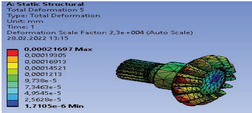
Figure 16 Deformation axle gear
