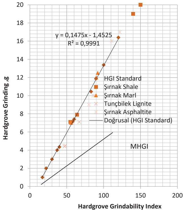
Figure 7. HGI Chart and Modified HGI at 10 min Microwave radiated materials studied.
