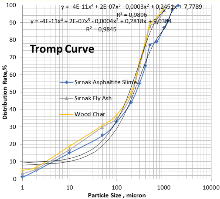
Figure 6. Particle size distribution of Hydrocyclone Decantation circuit for Oily Froth Overflow.
