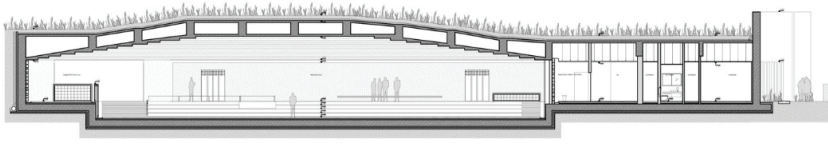
Figure 5: Section showing the green roof of the Sancaklar Mosque. (Url-2)
