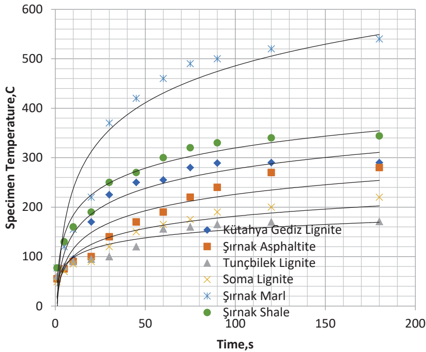
Figure 5. The microwave radiated pellet temperature changes of grinding materials prior to finer grinding to under 20 micron
