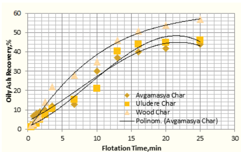
Figure 8 Char carrier cycling column flotation washing results with 10 % weigh rate fly ash use
