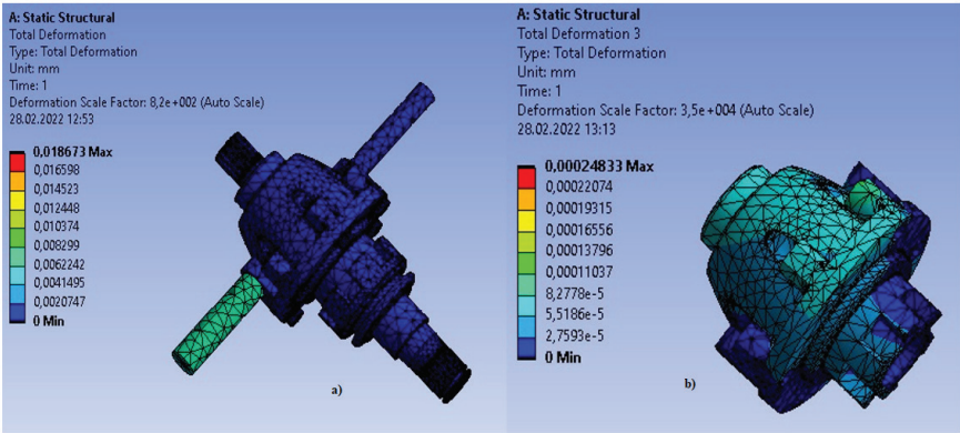
Figure 13 Total deformation a) Assembly and b) Main body
