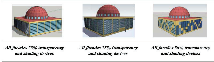
Figure 6 (continued): Different facade scenarios. (Zorer Gedik et al., 2021, p. 7)
