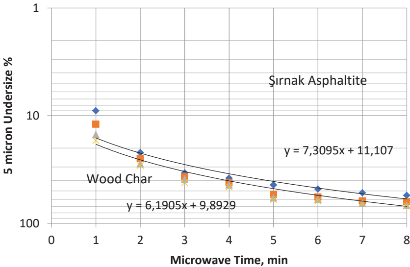
Figure 9. The Bij Breakage rate change for -5µm finer grinding at 30 min.
