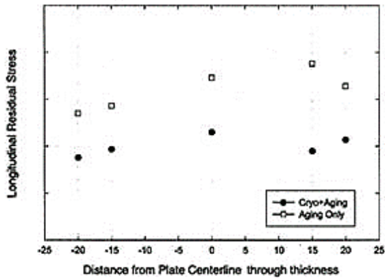
Figure 6. Longitudinal residual stress profiles of aluminum alloy (Chen et al., 2001).
