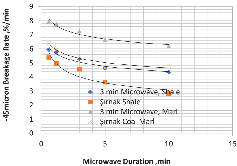
Figure 6. The breakage rate of Şırnak quarry shale 45 \mu m under Microwave Interaction
