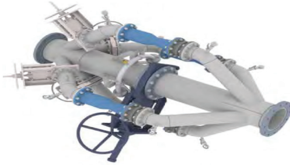
Figure 2. Pumping cavity circulated Aeration of slurry in Column Flotation tank (Eriez Company)[23]
