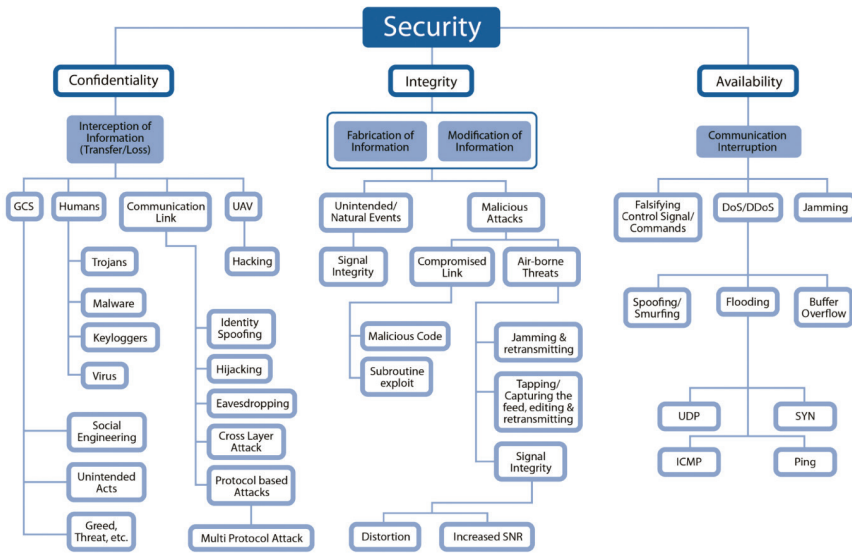
Fig 6. UAV Security
