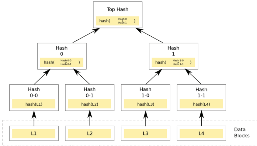
Fig 4. Merkle Tree
