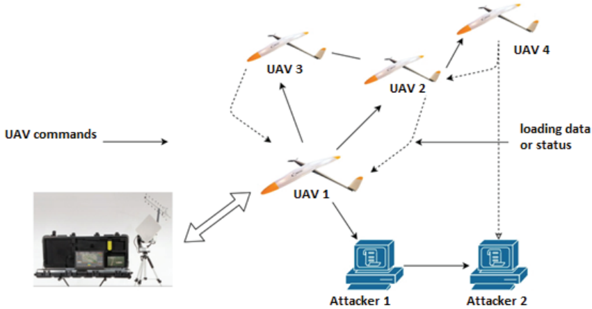
Fig 8. Wormhole Attack
