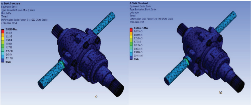
Figure 10 a) Equivalent Stress Analysis b) Equivalent Elastic Strain
