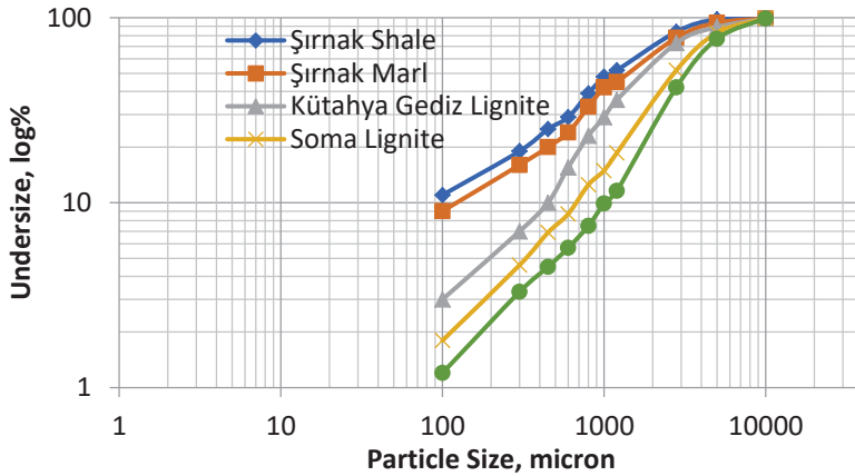
Figure 3. Şırnak Asphaltite, marl and shale samples of Gaudin Schumann Particle Size Distribution.
