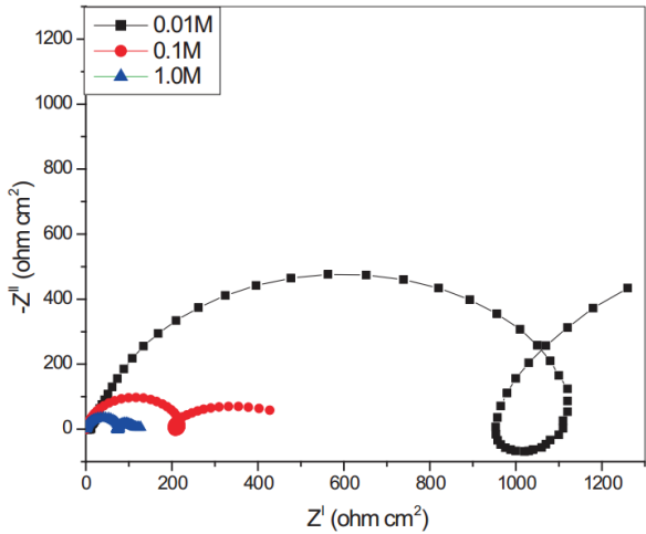
Figure 11. The Nyquist curves of 6063 alloy in different concentration of H_3PO_4 at 30 °C (Deepa & Padmalatha, 2017).
