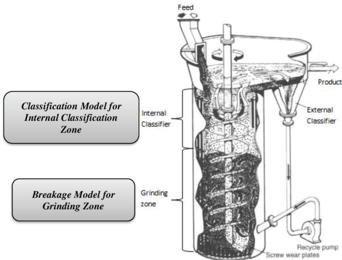
Figure 1. The vertical ball mill model [5-6]
