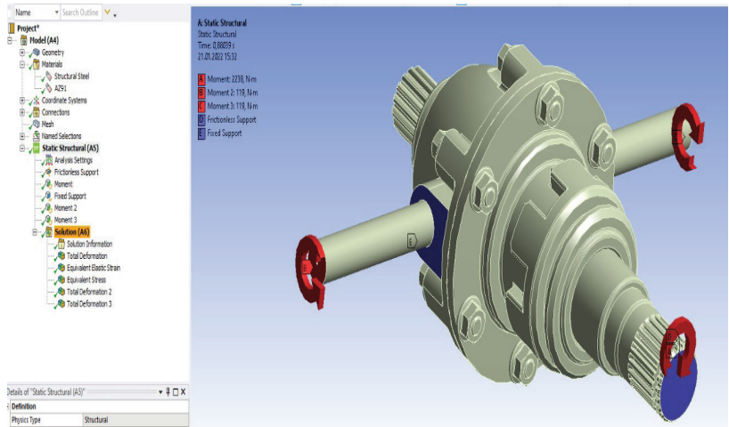
Figure 8 Torques in the differential box
