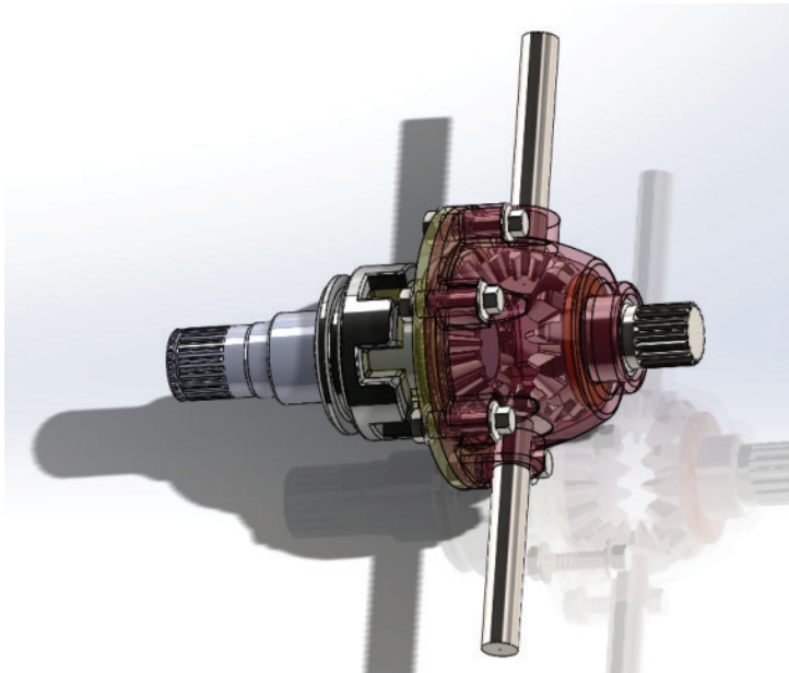
Figure 6 Assembly Picture
