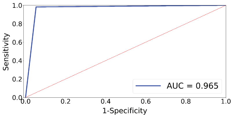
Figure 5. ROC curves of the proposed model
