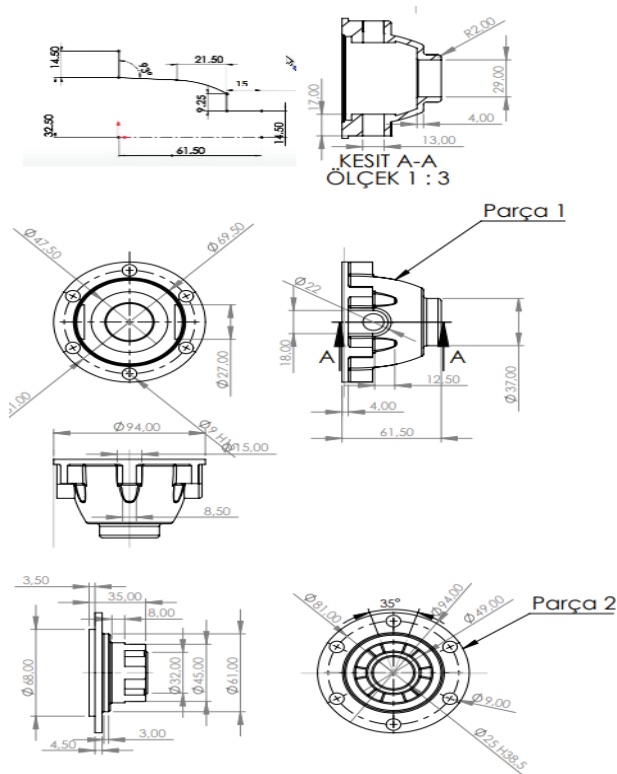
Figure 2 Dimensioning of the Drawing
