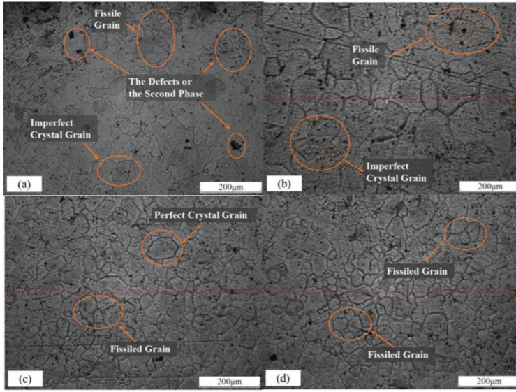
Figure 5. 2024-T351 aluminum alloy; microstructure images a) untreated, b) CT-2h, c) CT-6h and d) CT-12h (Zhou et al., 2016).
