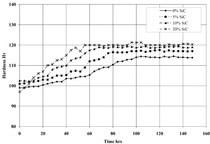
Figure 12. The hardness behaviour of composites (Bekheet et al., 2002).
