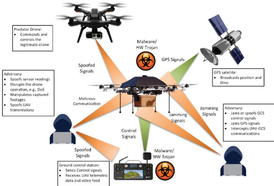
Fig 7. UAV Security Attack
