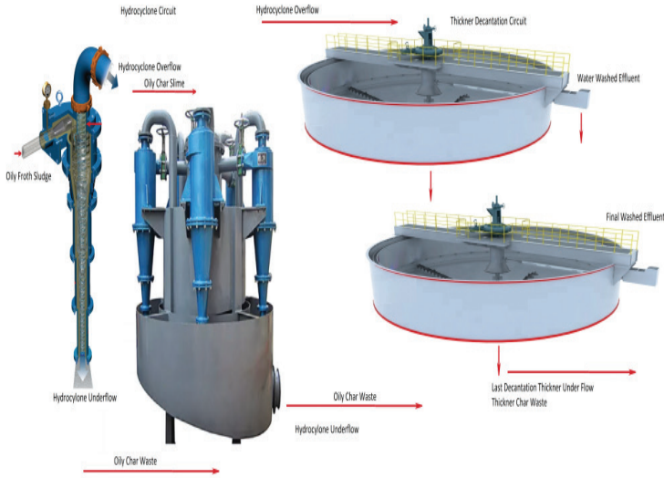
Figure 5. Decantation circuit, equipment for Oily Froth washing.
