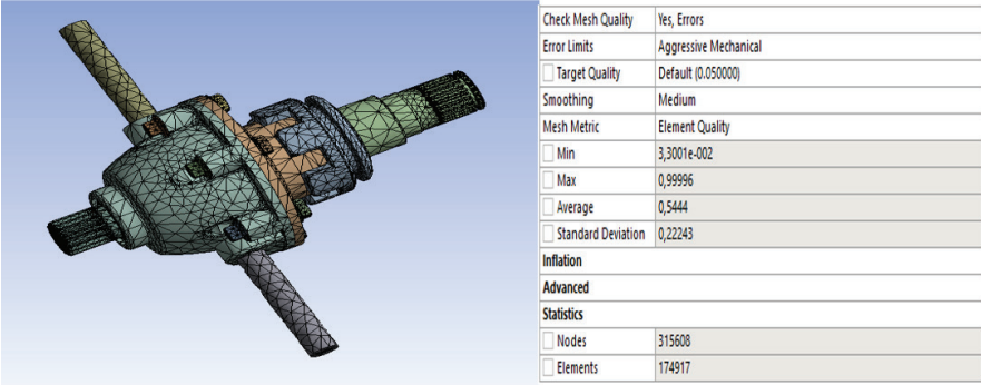
Figure 7 Finite Element Model of Differential Box
