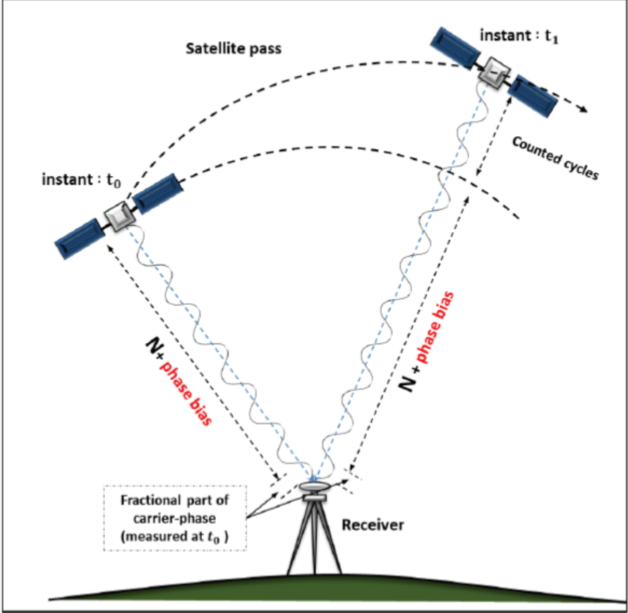
Figure 1. Geometric representation of ambiguities and carrier phase biases in carrier phase measurements over a satellite pass (Oliveira, 2017).
