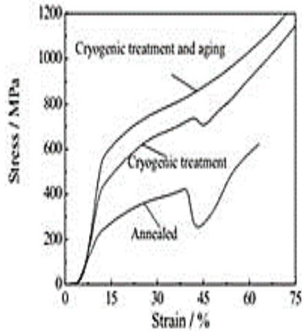
Figure 7. Untreated and treated LC4 (Al-Zn-Mg-Cu) alloy compression test results.
