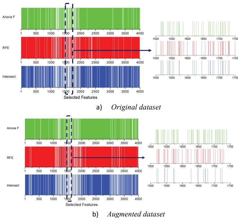
Figure 4. Graphical representation of features selected from ANOVA F value and RFE methods and intersected features
