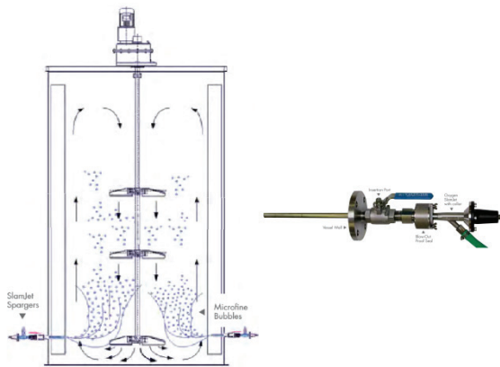
Figure 2. Jet Gas Aeration of slurry in Column Flotation tank (Eriez Company)[23]
