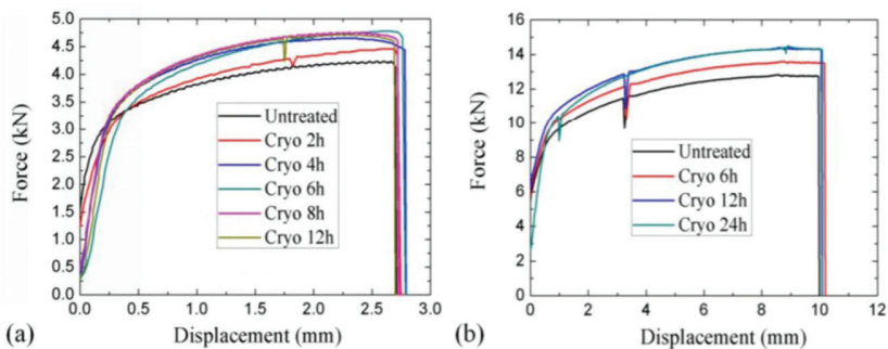
Figure 4. 2024-T351 aluminum alloy tensile curves; a) N1-0-N1-5 b) N2-0-N2-3 (Zhou et al., 2016) .
