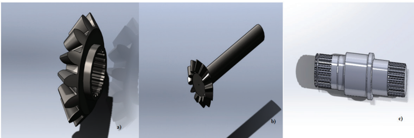
Figure 5 a) Hollow bevel gear b) Pinion gear c) Shaft
