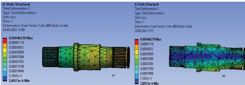
Figure 15 Deformation a) axle shaft b) axle shaft section
