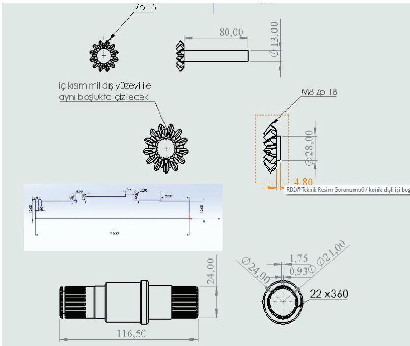
Figure 3 Dimensioning the Drawing (continued)
