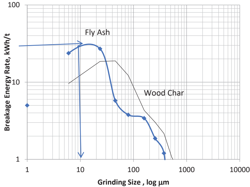
Figure 11. Breakage Energy Change by the microwave interacted fly ash and wood char samples.
