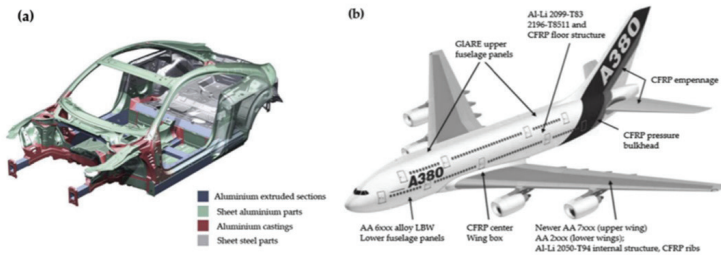
Figure 1. Aluminum use in automotive and aviation a) Audi TT coupé and b) A380 (Zheng et al., 2018).
