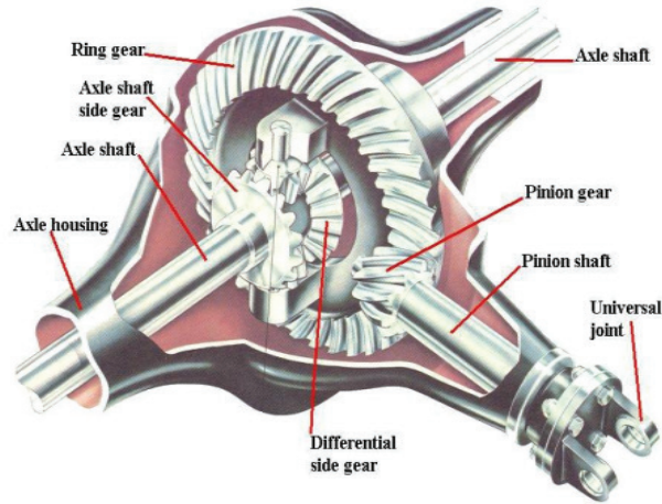
Figure 1. Parts of the Differential Gearbox (Singh, Kumar, kumar dewangan, kumar sen, & kumar bohidar, 2014)
