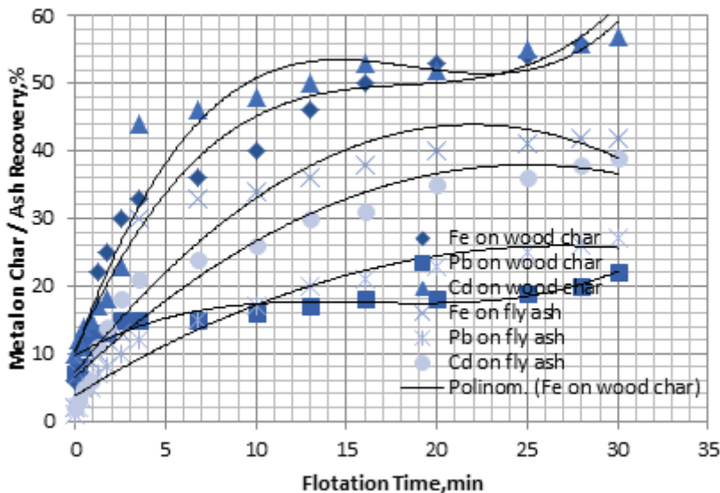
Figure 9. The wood char cycling column flotation washing results
