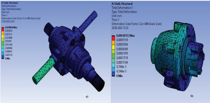
Figure 9 Total deformation a) Assembly and b) Main body
