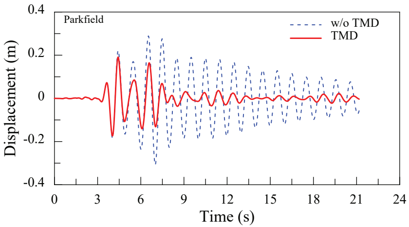
Fig. 7. Time histories of the top story displacement.
