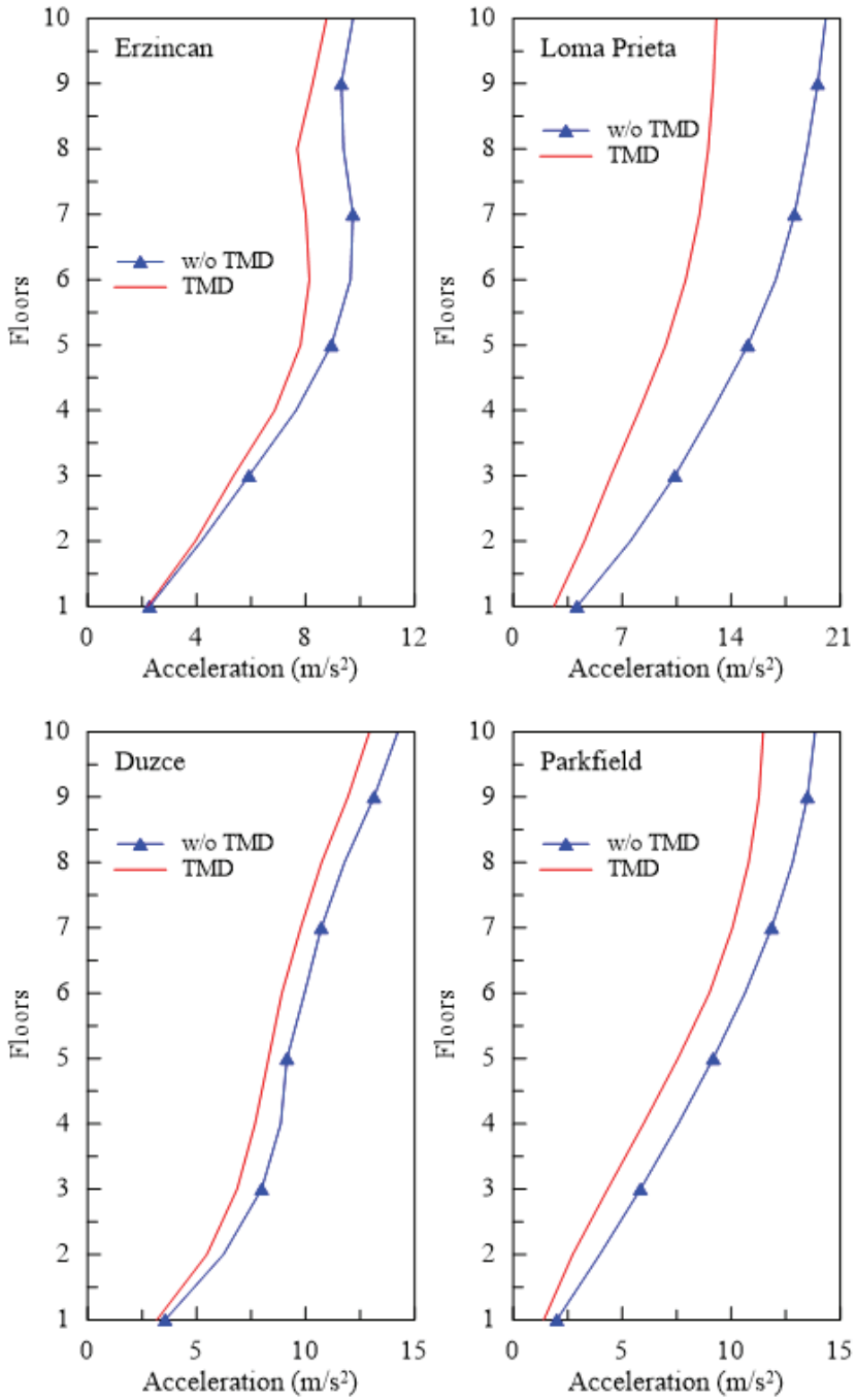
Fig. 6. The maximum acceleration of floors under various earthquakes.
