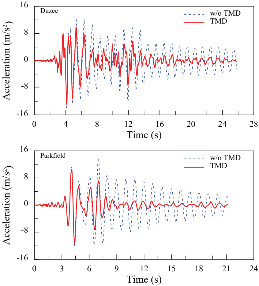
Fig. 8. Time histories of the top story acceleration.
