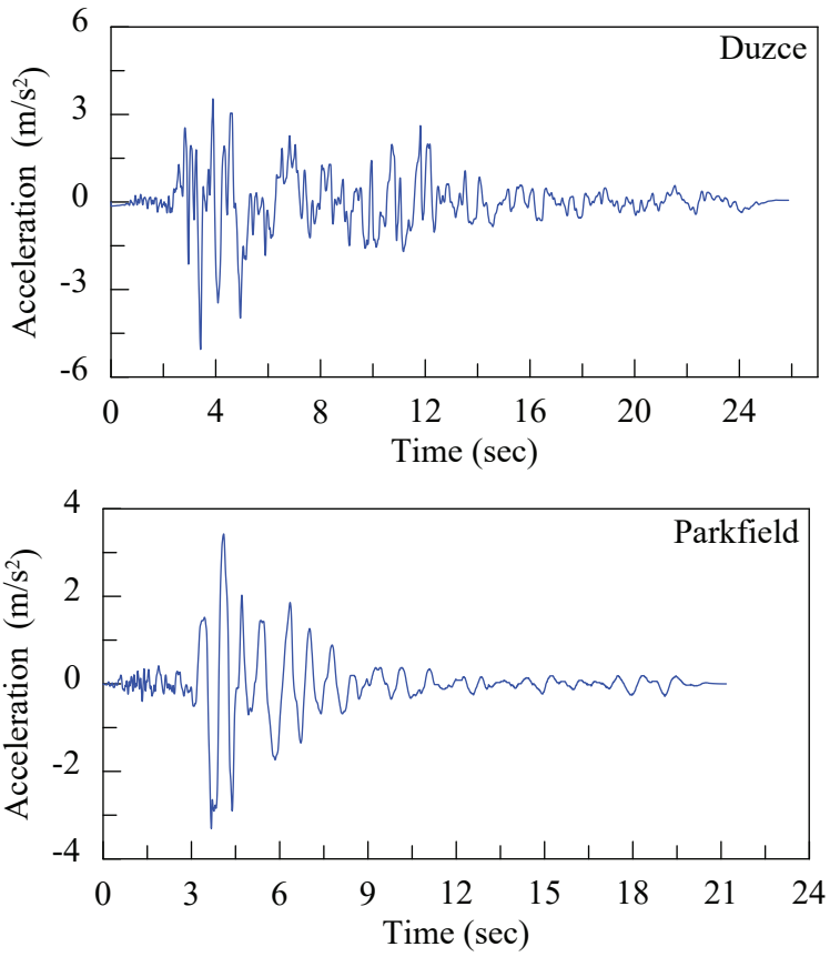
Fig. 4. The acceleration record of the selected earthquakes.
