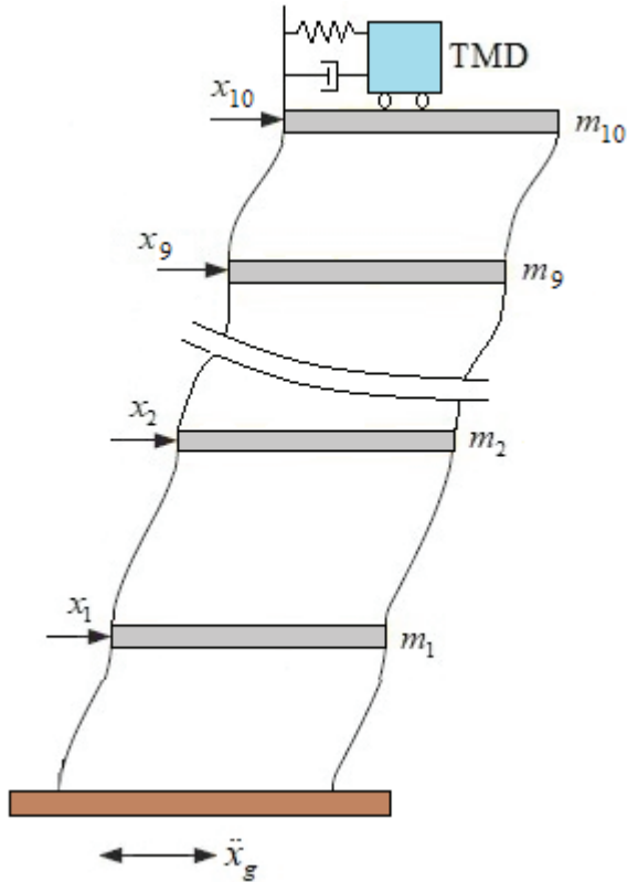
Fig. 1. Ten-story shear building with TMD.
