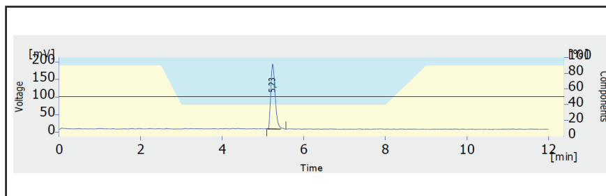
Figure 4. HPLC-UV chromatograms of of [^{68}\text{Ga}]^{68}\text{Ga} -DOTATATE R_t = 5.23 min method: Mobile phase: 0,1% trifluoroacetic acid (TFA) in water (A) and 0,1% TFA in acetonitrile (B) gradient method 10-30% (B) in 10 min, Agilent C18 column, The injection volume 20 \mu\text{L} .
