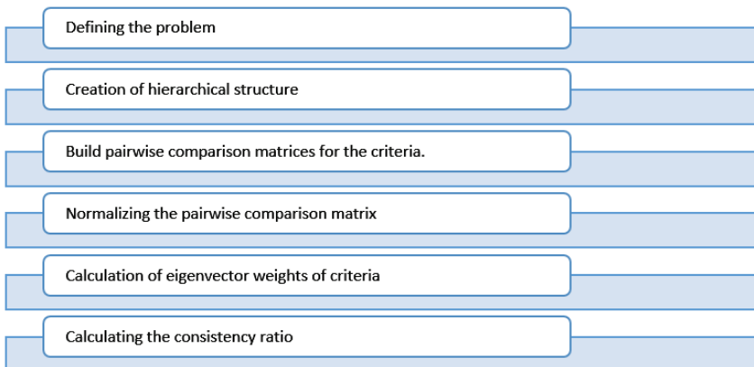
Figure 2. AHP Steps
