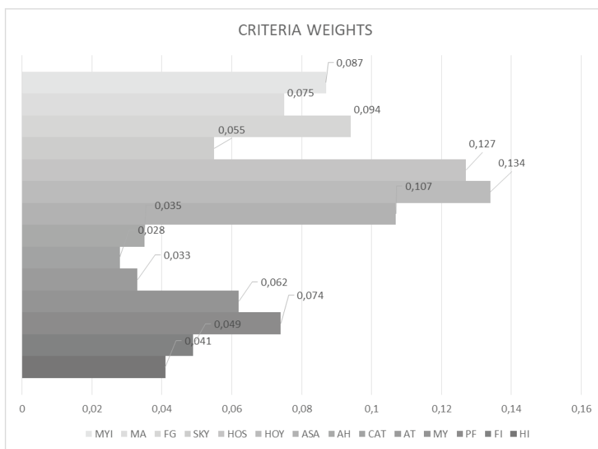
Figure 4. Bartın Province Criterion Weights
