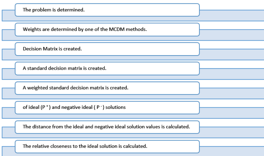
Figure 3. TOPSIS Steps
