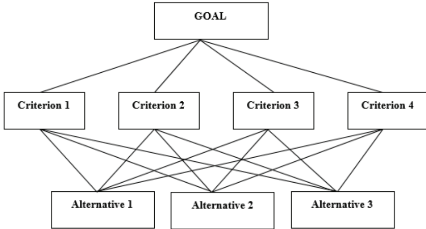
Figure 1. AHP Hierarchical Structure(Saaty,1980)
