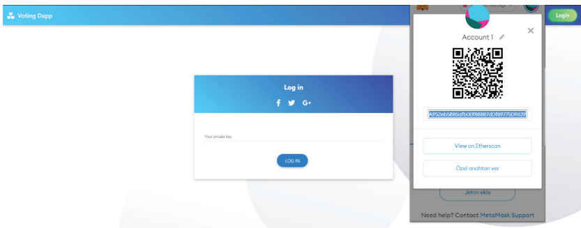
Figure 7. Login Page
