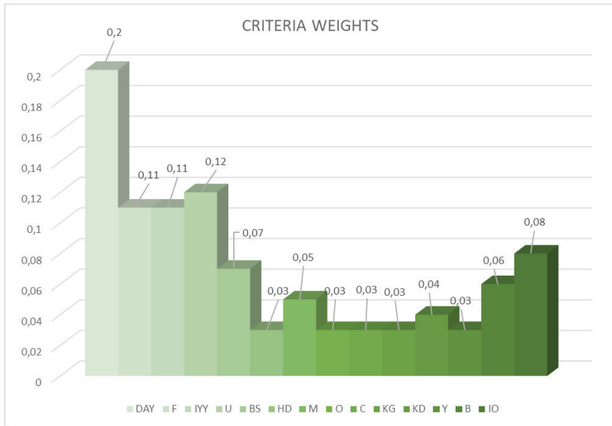
Figure 4. Istanbul Province Criterion Weights
