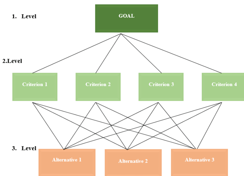
Figure 1: AHP Hierarchical Structure(Saaty,1980)
