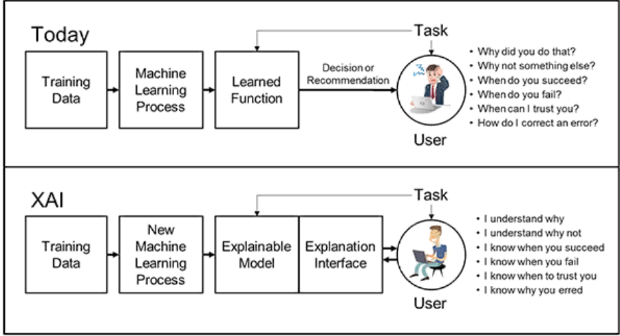
Figure 2. XAI Concept
